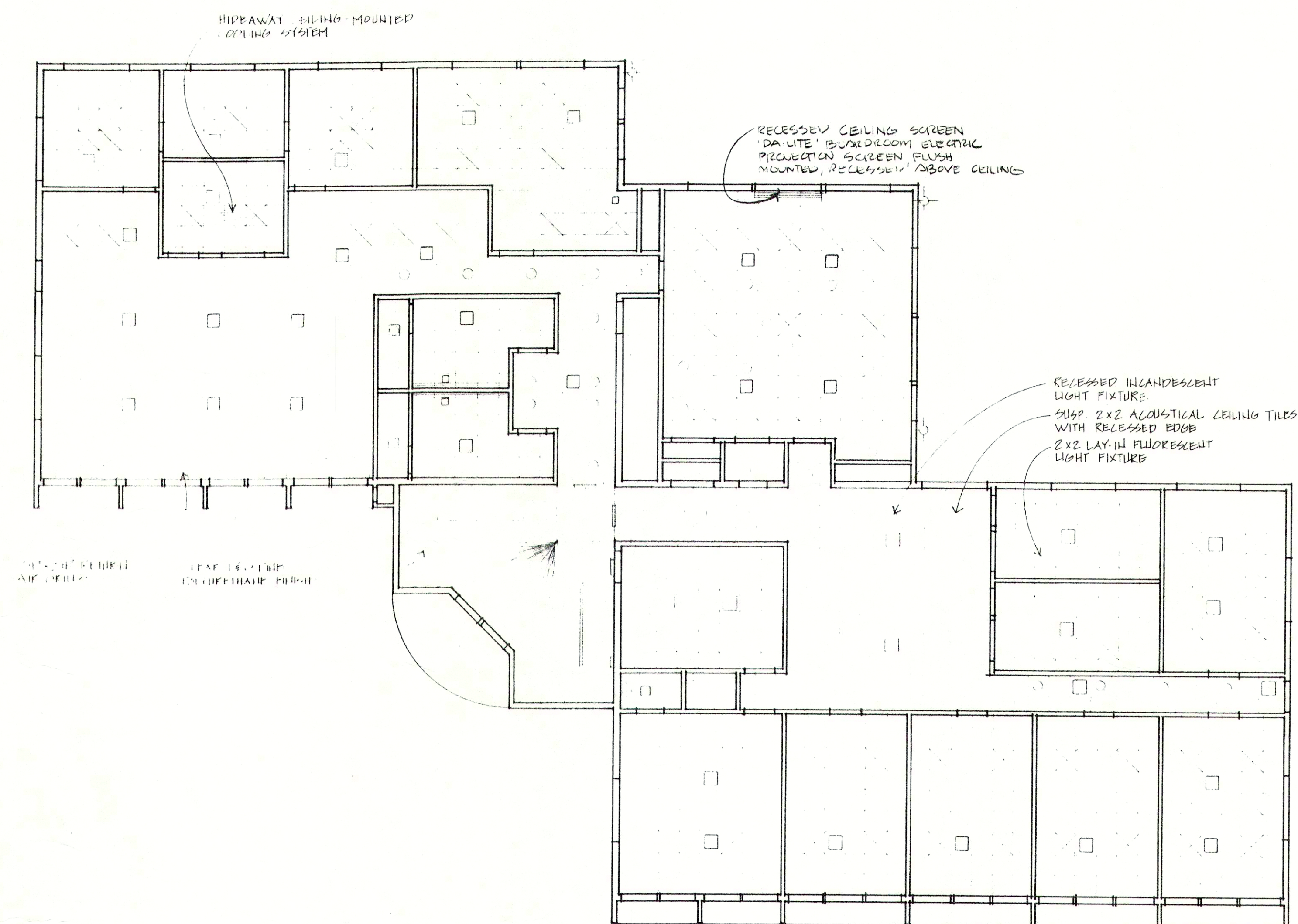
PI REFLECTED CEILING PLAN SCALE: 1/8" = 1'-0"
